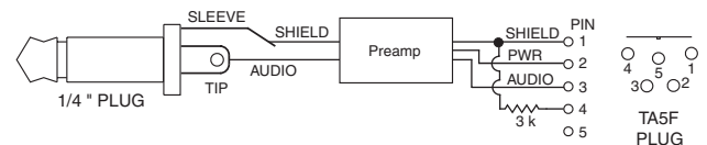
Simplified diagram of MI33AST cable assembly
