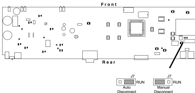
Figure 10 - Location of DC Bypass Jumper
