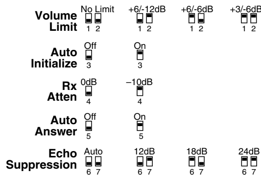
Figure 7 - TH2 Dip Switch Settings
