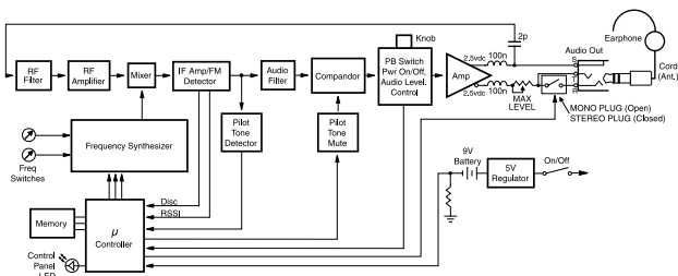
Figure 4 - R1a Block Diagram
