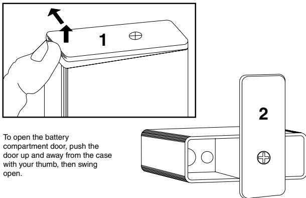
Figure 5 - Battery Replacement
